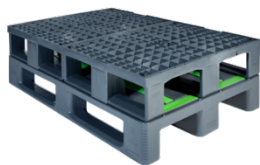
Fits to the Heilbronn Half-Pallet
